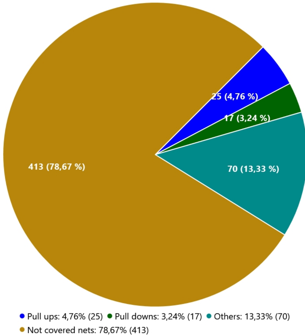
Figure 2: The complete test coverage overview for device: S32G275A
